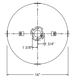
Mounting Plate Dimensions
