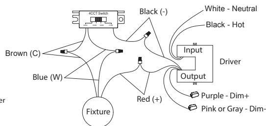
Fig.3 Driver Wires
