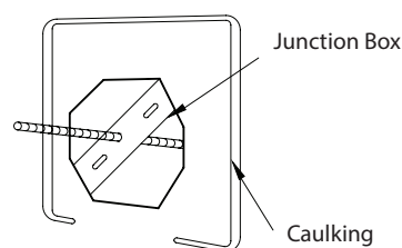
Fig. 3 Sealing
