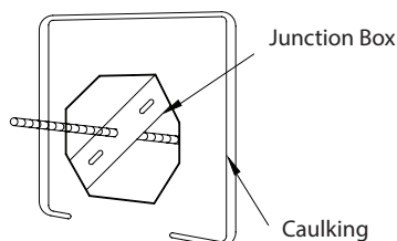
Fig. 3 Sealing
