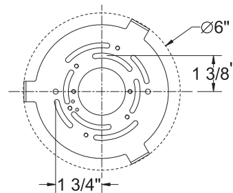
Back plate Dimensions
