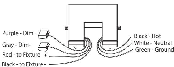
Fig. 3 Driver Wires
